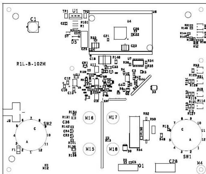
Figure 3: Parts Layout
