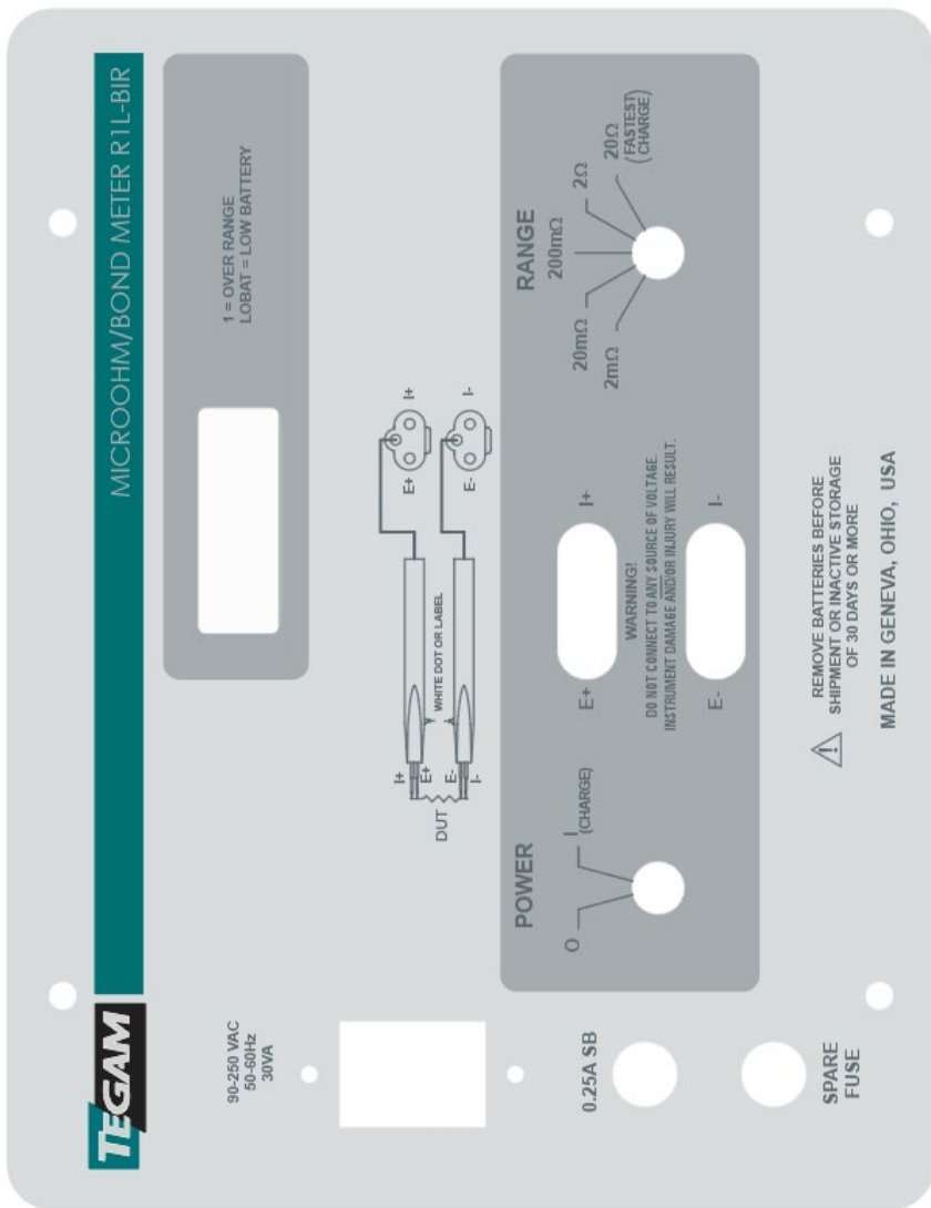
Figure 2b: R1L-BIR Front Panel Controls
